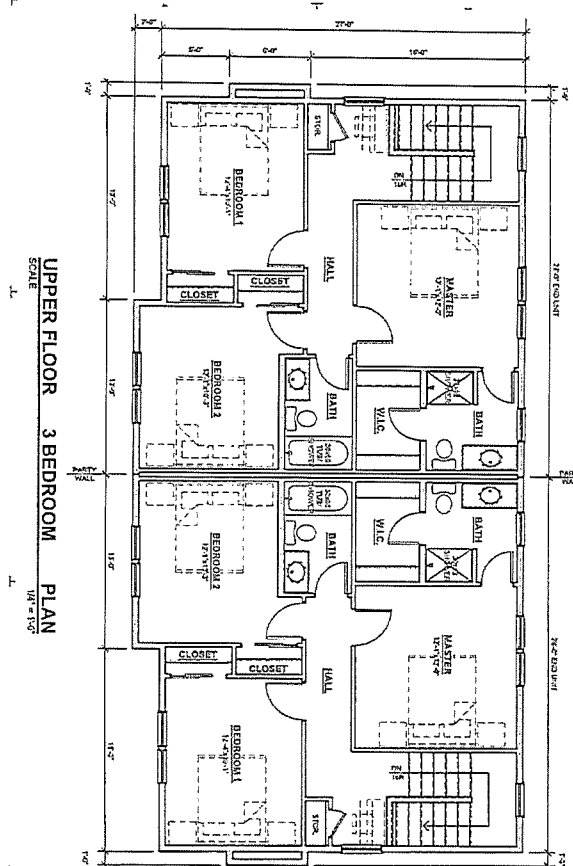
MAIN FLOOR 3 BEDROOM PLAN SCALE: 1/8" = 1'-0"
